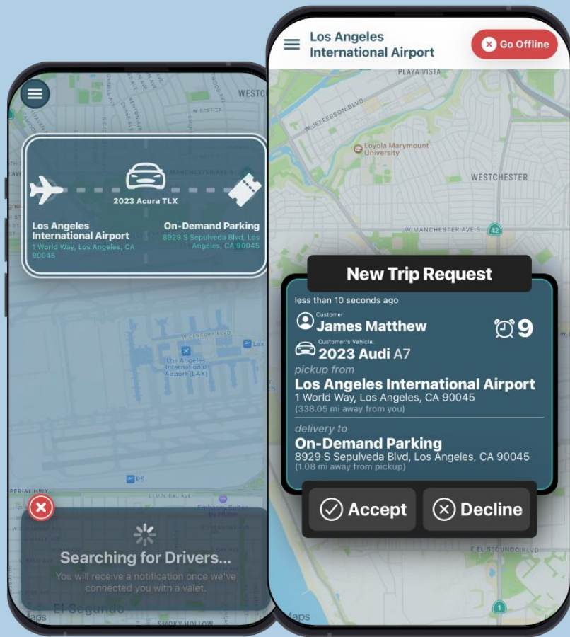
User App
